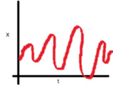
Non-Stationary series
